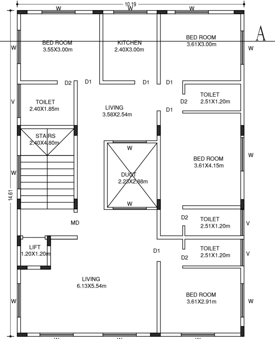
PROPOSED TYPICAL FIRST & SECOND FLOOR PLAN
